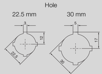
Holes are centered on the cover
